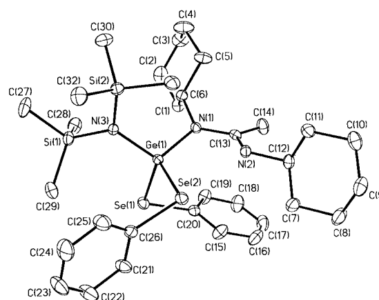
Fig. 2 Molecular structure for one of the independent molecules of [C 6 H 11 NC(Me)NC 6 H 11 ][Ge[N(SiMe 3 ) 2 ][SeC 6 H 5 ] 2 ( 13 ). Hydrogen atoms have been omitted for clarity. Thermal ellipsoids are drawn at 30% probability.
