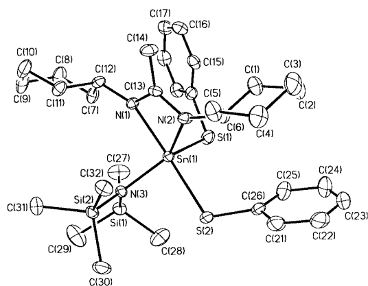
Fig. 3 Molecular structure for one of the independent molecules of [\text{C}_6\text{H}_{11}\text{NC}(\text{Me})\text{CN}_6\text{H}_{11}]\text{Sn}[\text{N}(\text{SiMe}_3)_2][\text{SC}_6\text{H}_5]_2 ( 14 ). Hydrogen atoms have been omitted for clarity. Thermal ellipsoids are drawn at 30% probability.
