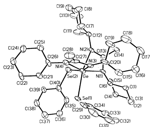
Fig. 1 Molecular structure of [\text{C}_6\text{H}_{11}\text{NC}(\text{Me})\text{NC}_6\text{H}_{11}]_2\text{Ge}[\text{SeC}_6\text{H}_5]_2 ( 10 ). Hydrogen atoms have been omitted for clarity. Thermal ellipsoids are drawn at 30% probability.
